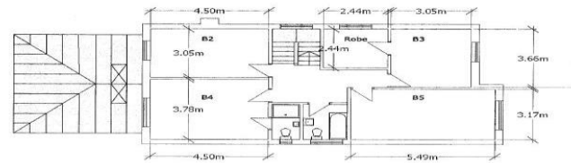
FIRST FLOOR
